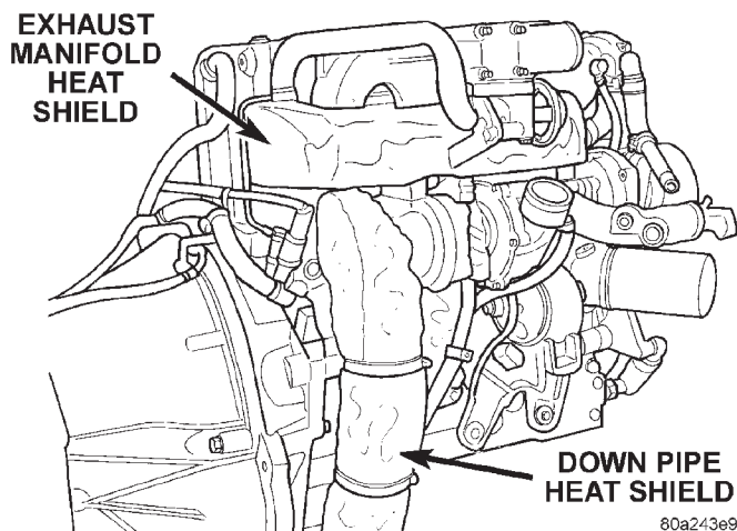
Fig. 1 Heat Shields
