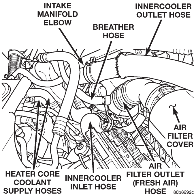
Fig. 4 Engine Compartment
